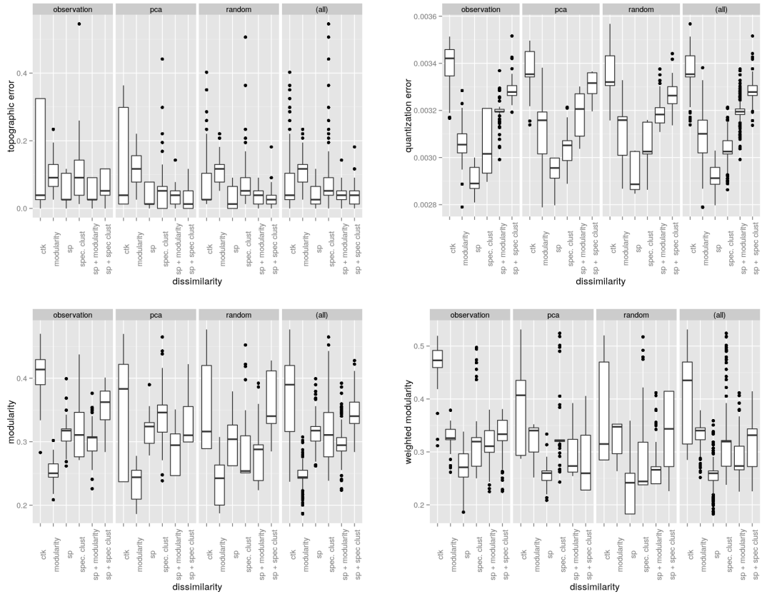
FIGURE 6. Distribution of the topographic and quantization errors and of the modularity (based on the weighted or unweighted) graph, given by dissimilarity and type of initialization. “clk” means “commute time kernel”, “sp” means “shortest path length” and “spec. clust” stands for the dissimilarity based on the eigen-decomposition of the Laplacian. “observations” means random initialization so that, for every u , \gamma_{ii}(u) = 1 for a unique i(u) , “pca” is the initialization based on a PCA-like approach and “random” is the initialization in which \gamma_{ii} are sampled in [0, 1] and then scaled such that \sum_i \gamma_{ii} = 1 . The last panel of each figure provides the distribution whatever the type of initialization (distribution over 3,000 maps).
